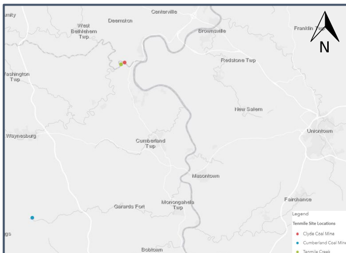
Figure 1. Map of southwestern Pennsylvania showing the sampling locations. Tenmile is the primary watershed within Greene County Pennsylvania, passing through Waynesburg before joining the Monongahela River in Clarksville, Pennsylvania.
